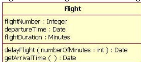
Figure 1: Class diagram for the class Flight
