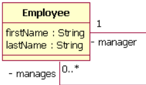
Figure 14: Example of a reflexive association relationship
