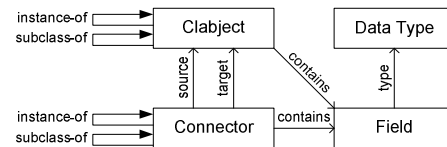
Figure 11. Language module entities
