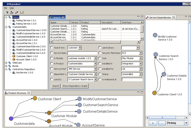
Fig. 7. Service Browser
